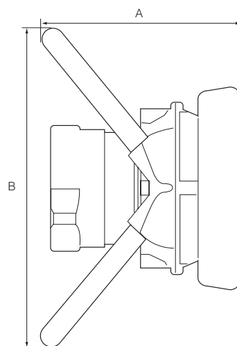
Medidas acople y adaptador. Coupler and adapter sizes.
